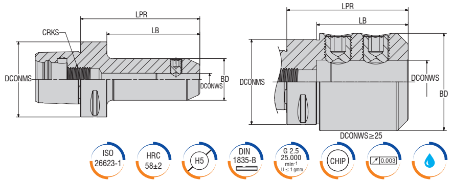
Dimensions in Metric
