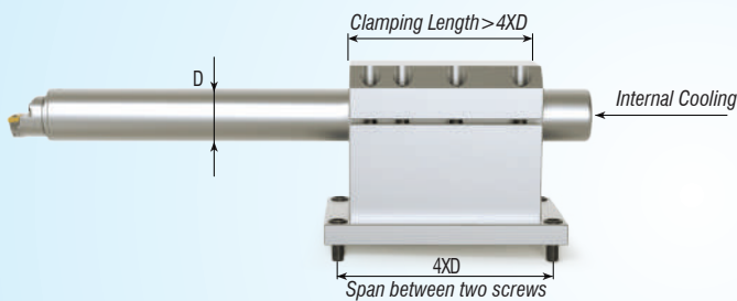
Type C Clamping method
